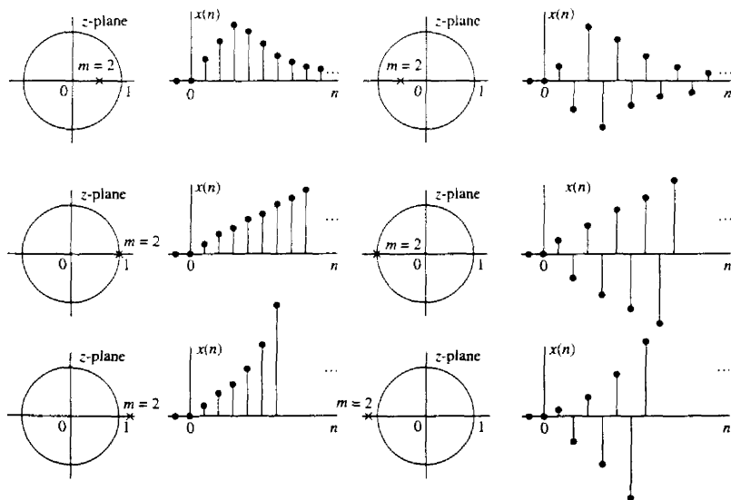
Figure 3.13 Time-domain behavior of causal signals corresponding to a double ( m = 2 ) real pole, as a function of the pole location.
